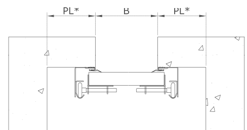
horizontal section
