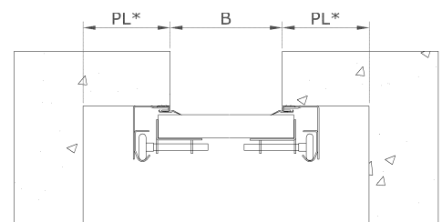
horizontal section
